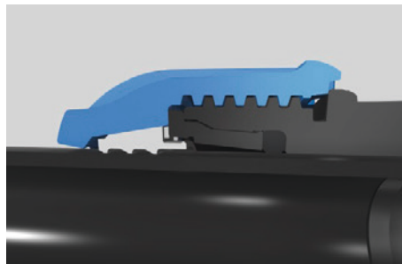
Connection cross-section
