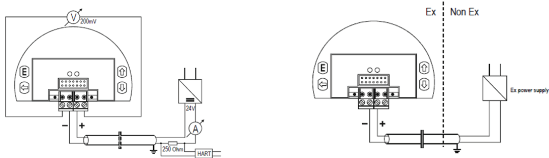
Standard wiring & connection of HART-Modem
