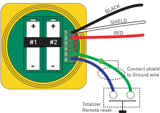
8150 Battery Powered Flow Totalizer
