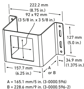
Heavy Duty Wall Mount Brackets (3-0000.596, 3-0000.596-1, 3-0000.596-2)
