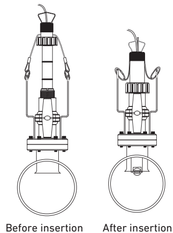
3519 Wet-Tap valve with a 515 Paddlewheel Sensor
