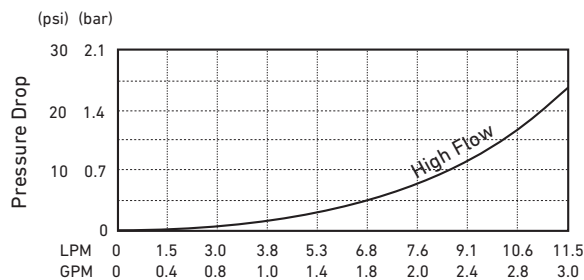
Model 2100 - High Flow
