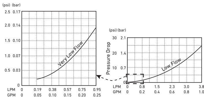
Model 2100 - Low Flow
