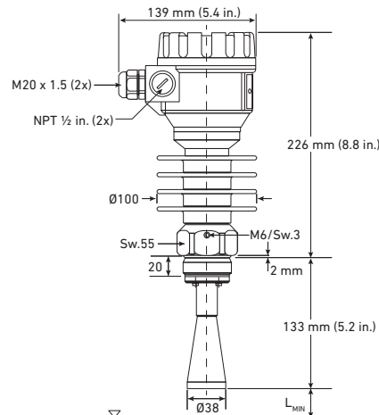
Stainless Steel 316 Ti horn antenna & temperature isolator Lmin: 200 mm (7.9 in.)
