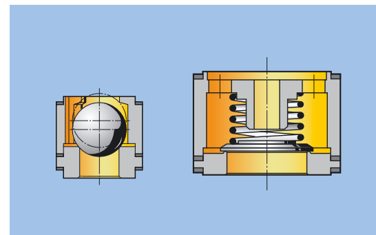
Low wear valves for various applications
